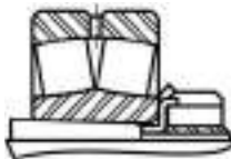
Fig. 12. Mounting with adapter sleeve
