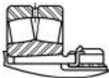
Fig. 13. Mounting with withdrawal sleeve
